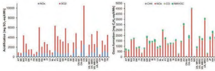
Figure 6 Estimated NO_x -, SO_2 -, CH_4 -, NMVOC -, NO_x -, and CO -Emissions of electric production in the various countries
