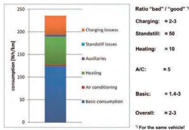
Figure 2 Possible contribution and range of electricity consumption in a battery electric vehicle
