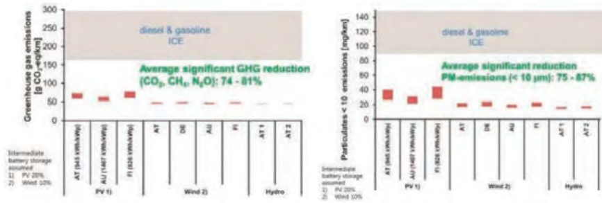
Figure 11 GHG- and PM (< 10 μm)-Emissions of Electric Vehicles - Renewable Electricity
