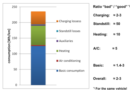
Figure 2: Possible contribution and range of electricity consumption in a battery electric vehicle [6]
