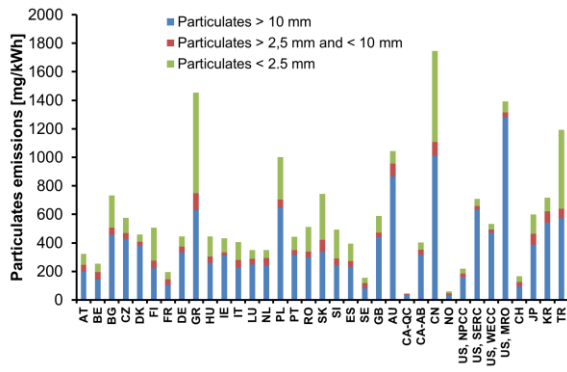
Figure 6: Estimated PM-Emissions of electric production in the various countries (mainly based on [8])
