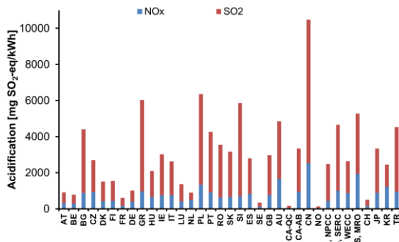
Figure 7: Estimated NO x – and SO 2 - Emissions of electric production in the various countries (mainly based on [8])
